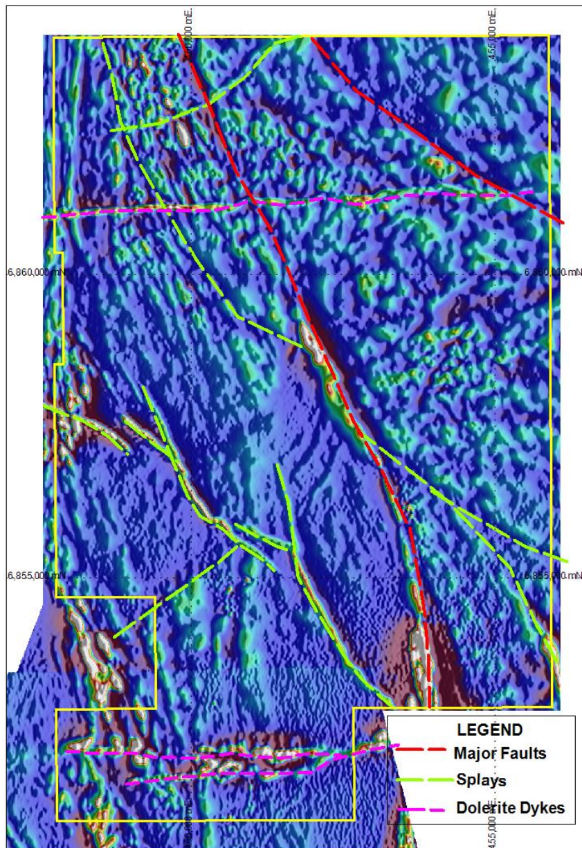
Figure 2 – Laverton Project Structural Interpretation from Magnetic Survey (RTP 1VD)
