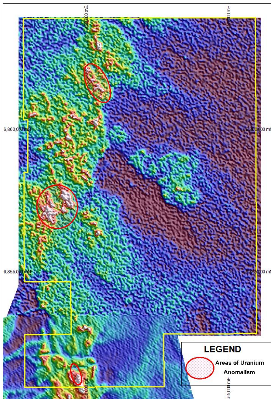
Figure3 – Laverton Uranium Anomalous Areas
